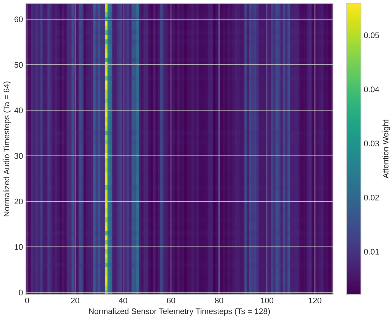
LACA Cross-Attention Matrix (Audio Query vs IMU Key)
